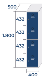
ECOC-40/1 PRO 25,7kg · 0,36m 3
